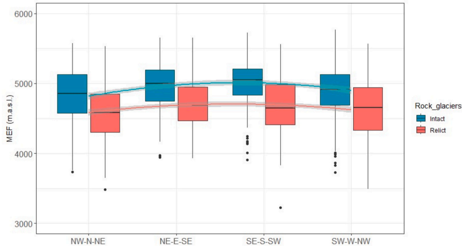
Fig. 4. Boxplots showing the distribution of intact (I-DLs) and relict rock glaciers (DDAs) across the Himalaya by aspect and elevation. The smooth lines display the polynomial regression models of mean MEF (m.a.s.l.) with aspect group for intact and relict glaciers. The polynomial regression model for the mean MEF and aspect of intact rock glaciers is:
